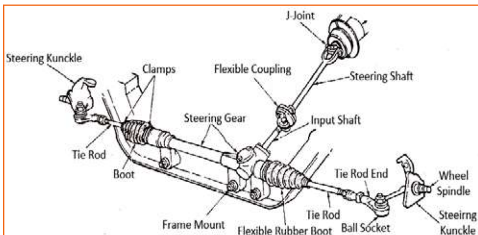
Fig 4.3.157: Rack and pinion steering system
