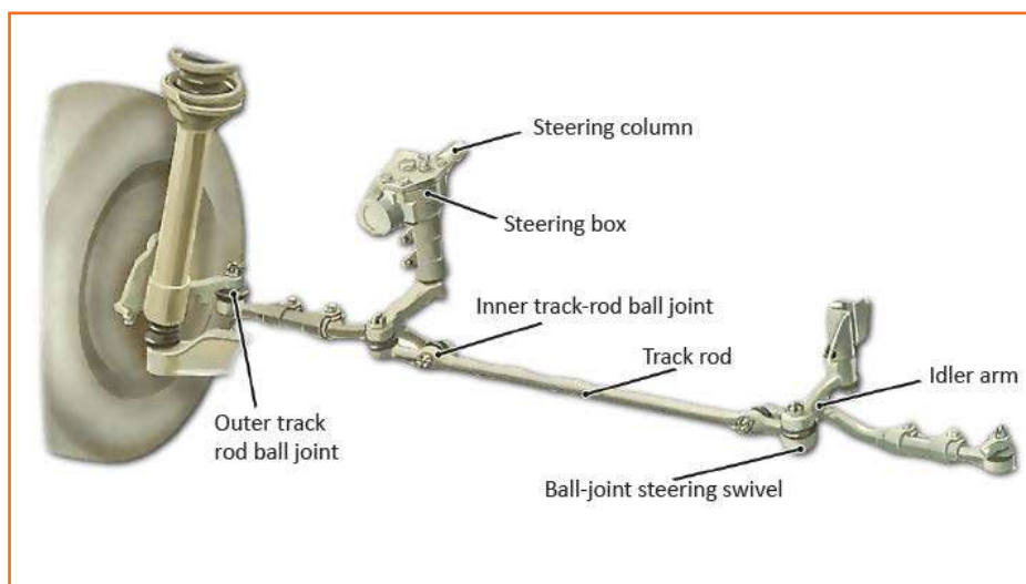
Fig 4.3.179: A Macpherson-strut suspension system with a steering box
