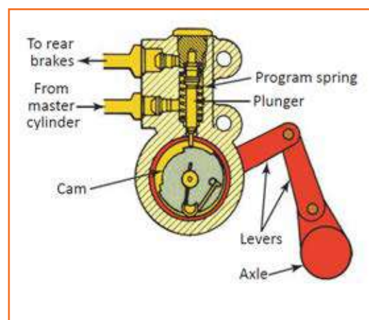
Fig 4.3.190: Load sensing pressure valve (LSPV)
