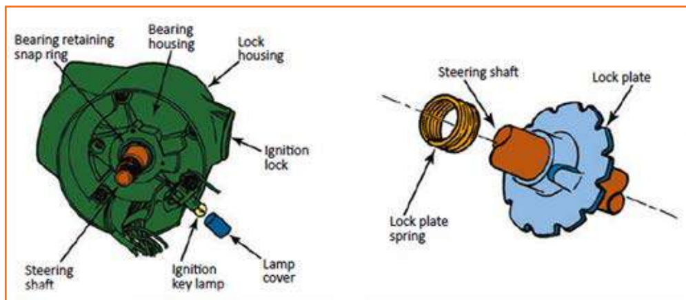
Fig 4.3.148: Upper section of steering column & lock plate
