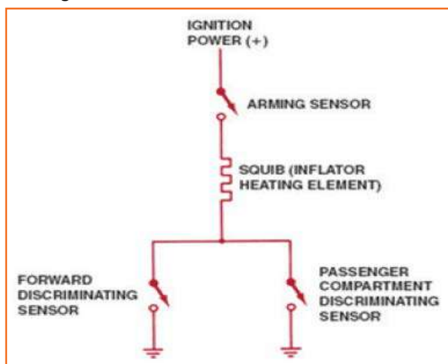
Fig 4.3.261: Air Bag Deployment Circuit
