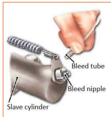
Fig 4.3.79: Fitting bleed tube
