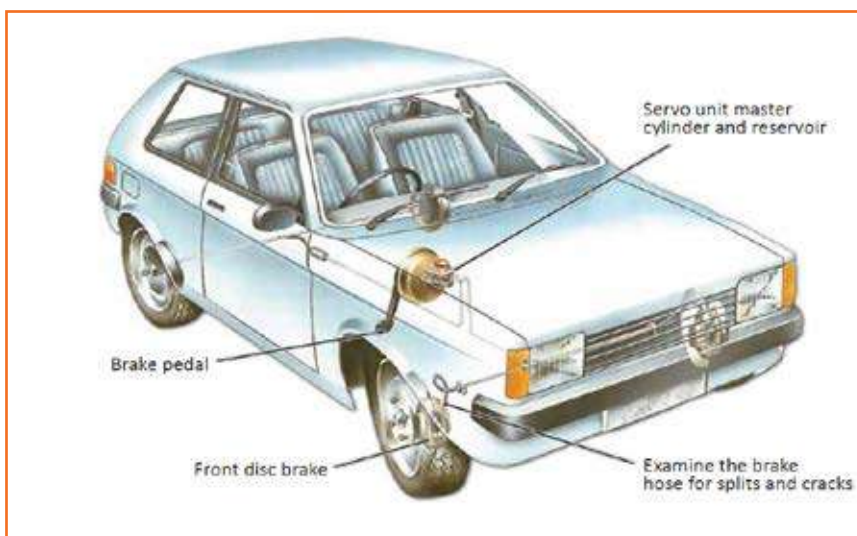
Fig 4.3.199: Break system
