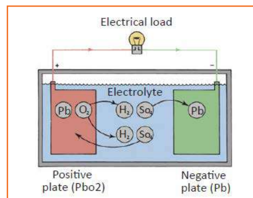
Fig 4.3.271: Working of battery
