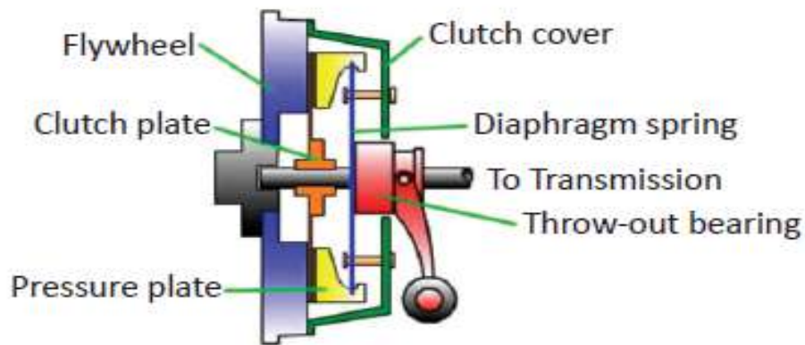
Fig 4.3.70: Clutch working
