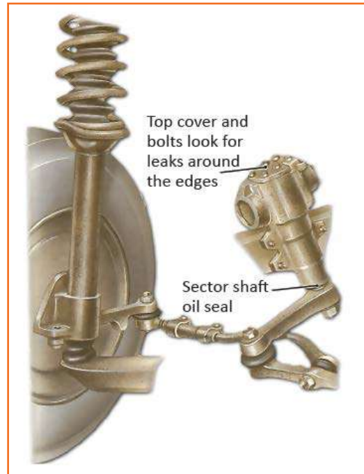
Fig 4.3.173: Checking steering box
