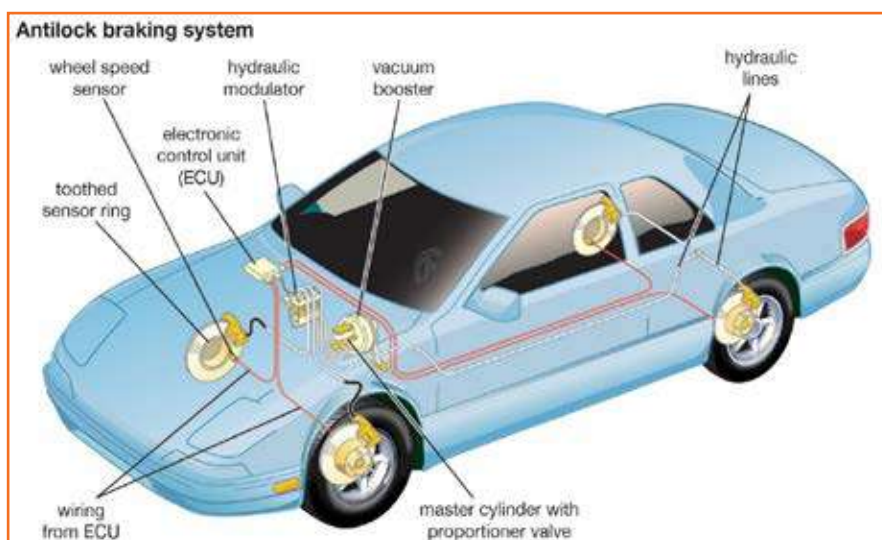
Fig 4.3.291: ABS system
