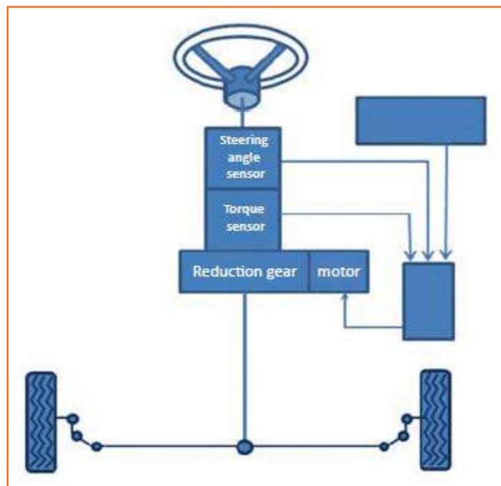
Fig 4.3.159: Electronic power steering
