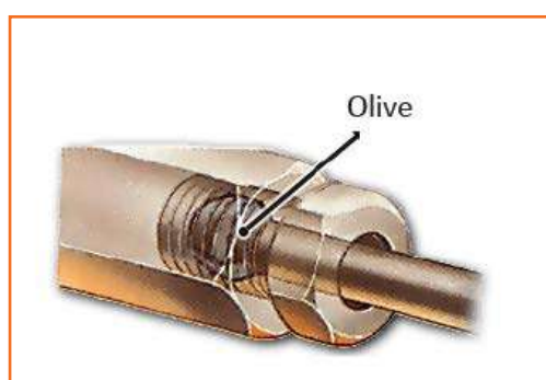
Fig 4.3.20: Metal pipe connection
