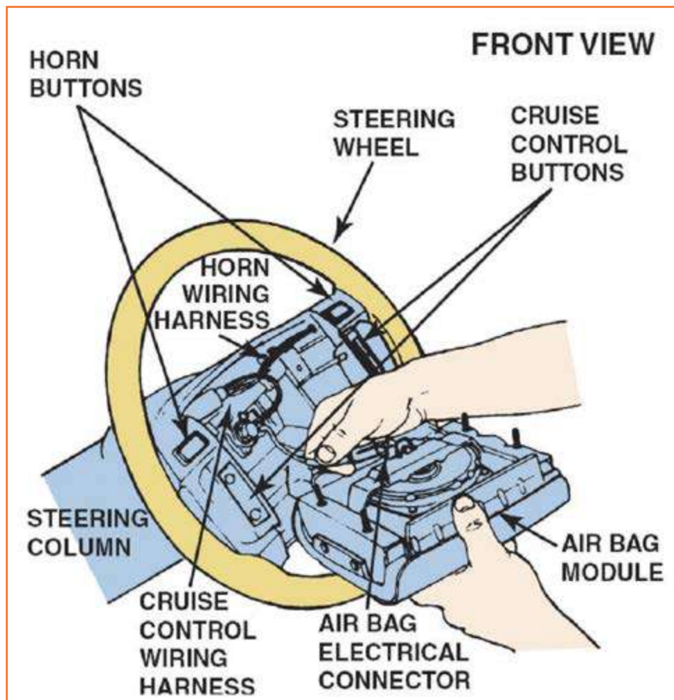
Fig 4.3.263: Airbag module replacement
