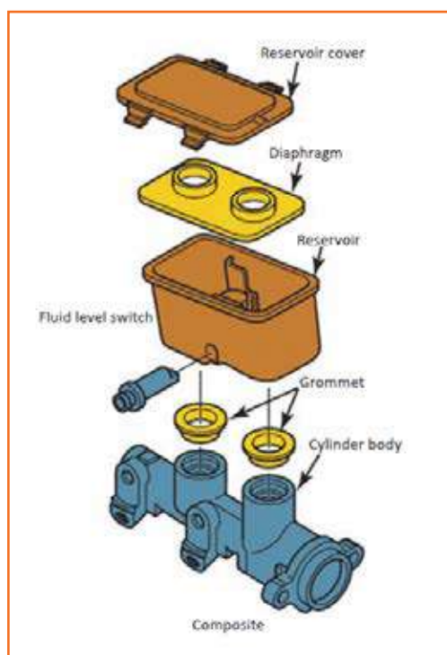
Fig 4.3.188: Components of master cylinder
