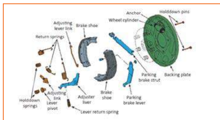
Fig 4.3.183: Drum brake assembly
