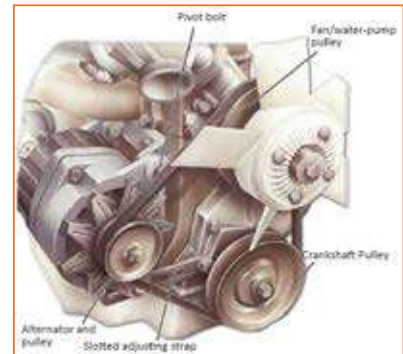
Fig 4.3.141: Drive belts
