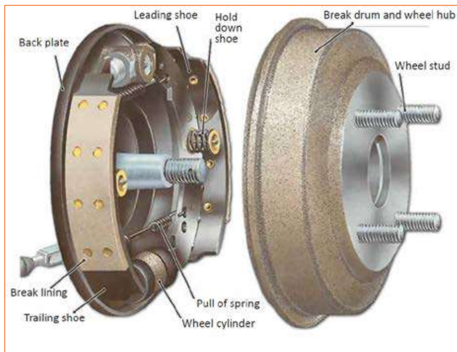
Fig 4.3.202: Integral drum brake
