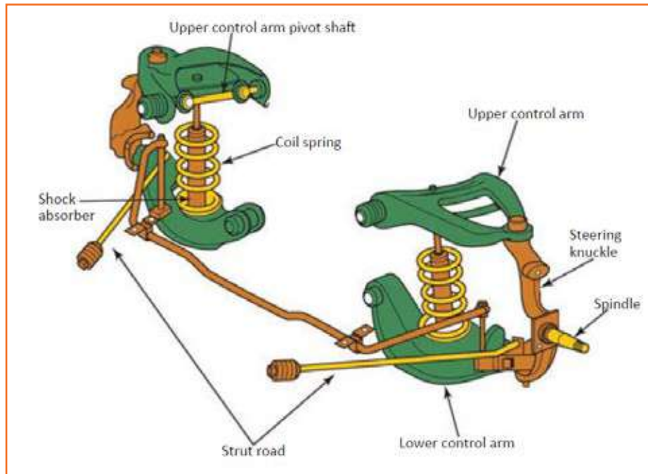
Fig 4.3.123: Strut Rods
