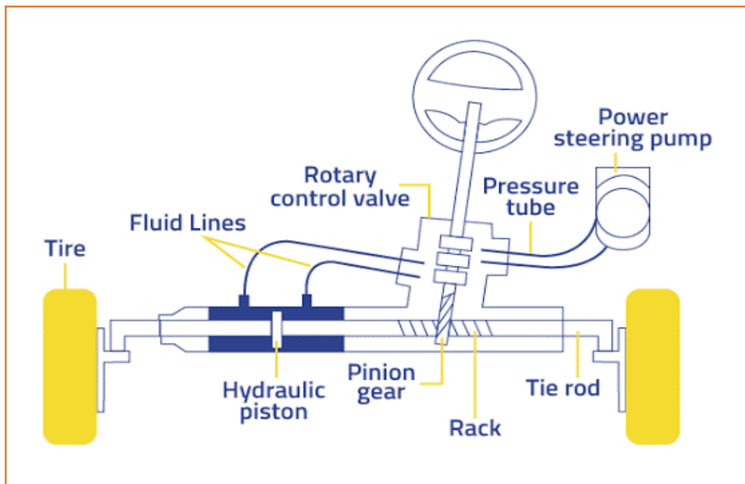
Fig 4.3.158: Components of hydraulic power steering
