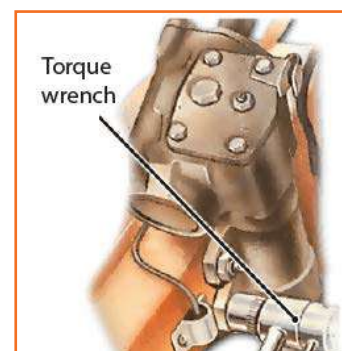
Fig 4.3.167: Steering mounting
