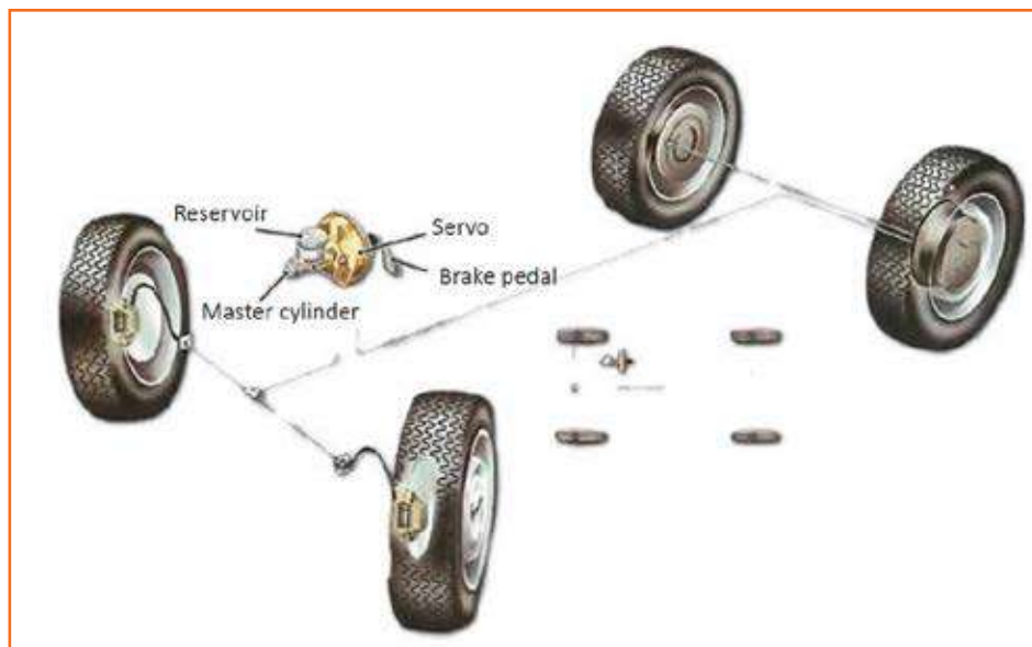
Fig 4.3.225: Bleeding a dual brake system
