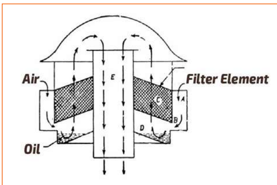
Fig 4.3.55: Oil bath type air cleaner
