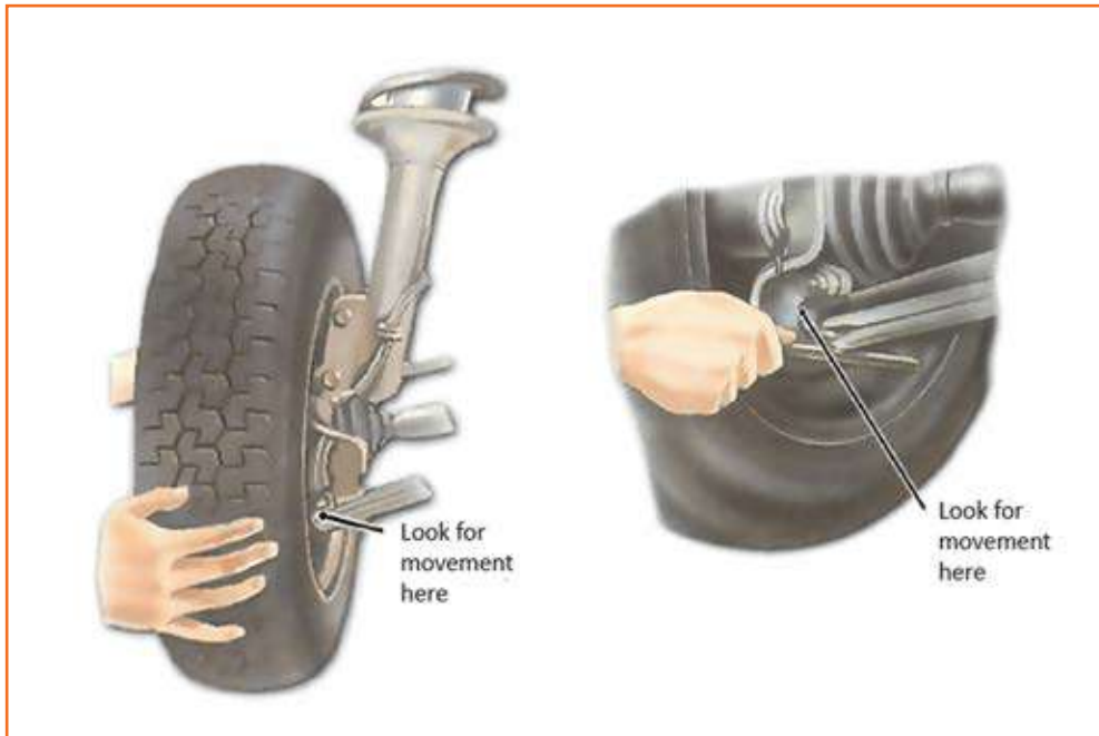
Fig 4.3.169: Macpherson strut check
