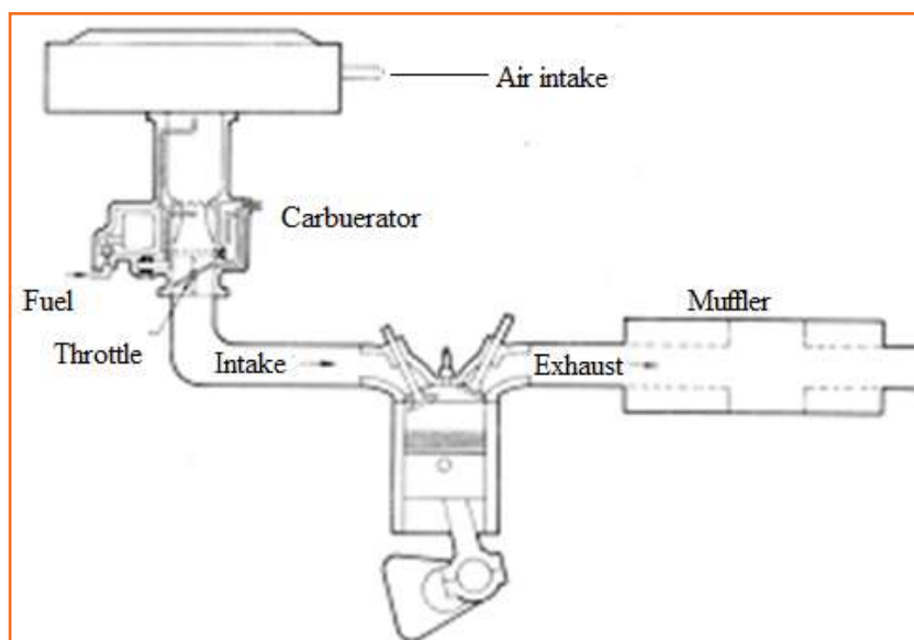
Fig 4.3.54: Exhaust system
