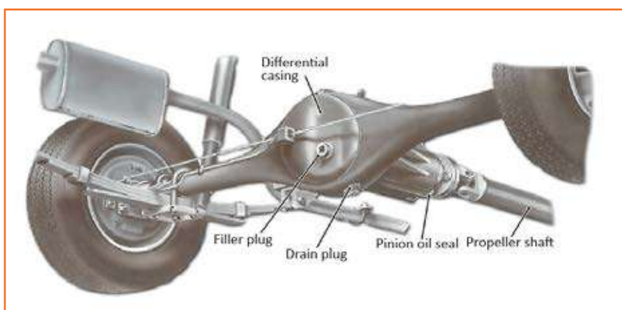
Fig 4.3.102: Parts of rear axle
