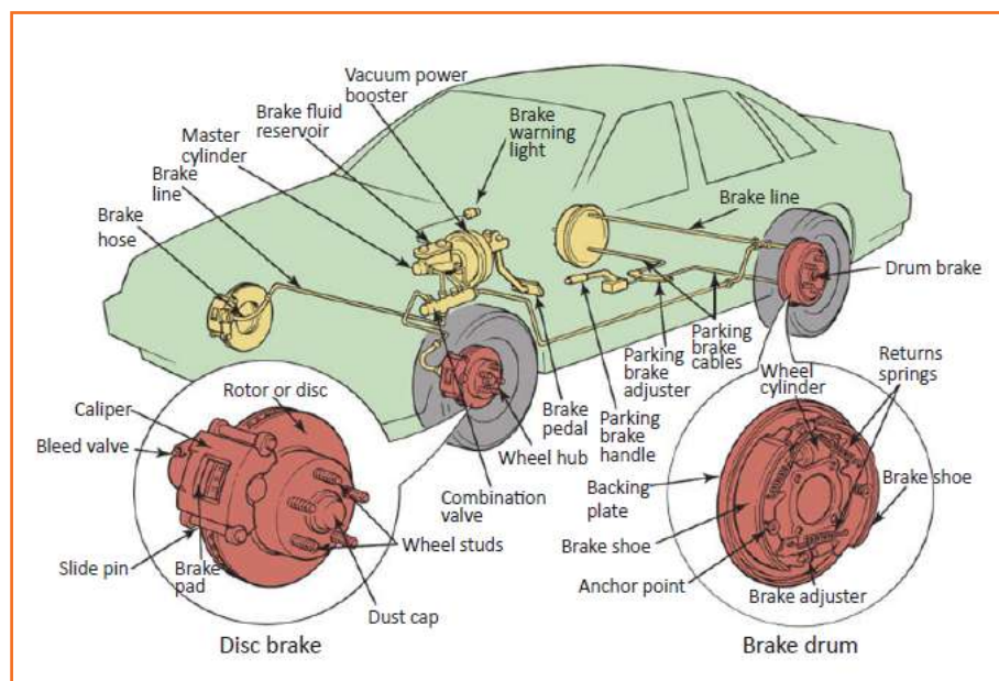
Fig 4.3.180: Brake system
