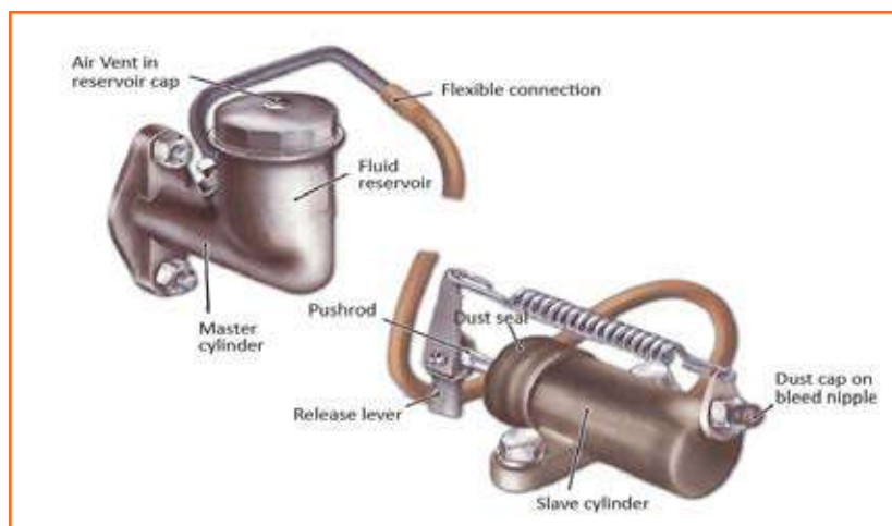
Fig 4.3.77: Clutch bleeding process
