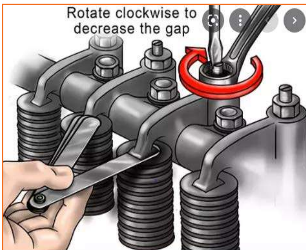
Fig 4.3.21: Tappet setting
