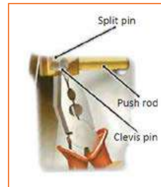
Fig 4.3.238: Disconnecting push rod
