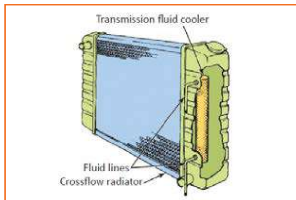
Fig 4.3.39: Transmission fluid cooler
