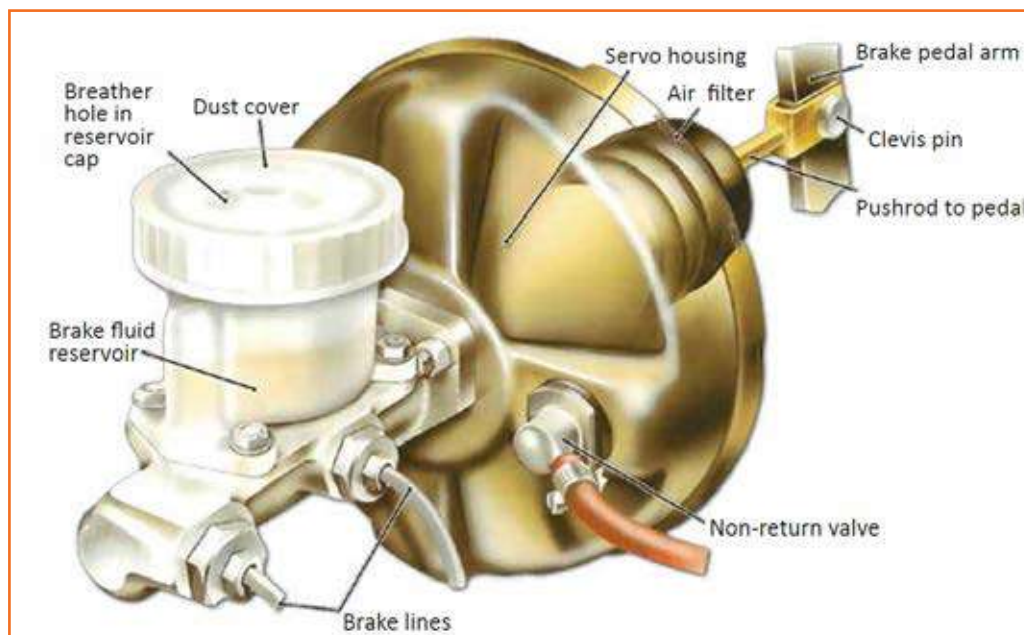
Fig 4.3.234: Dual circuit cylinder and servo
