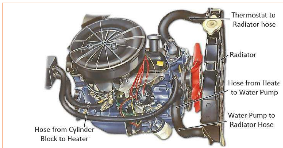
Fig 4.3.47: Parts of cooling system
