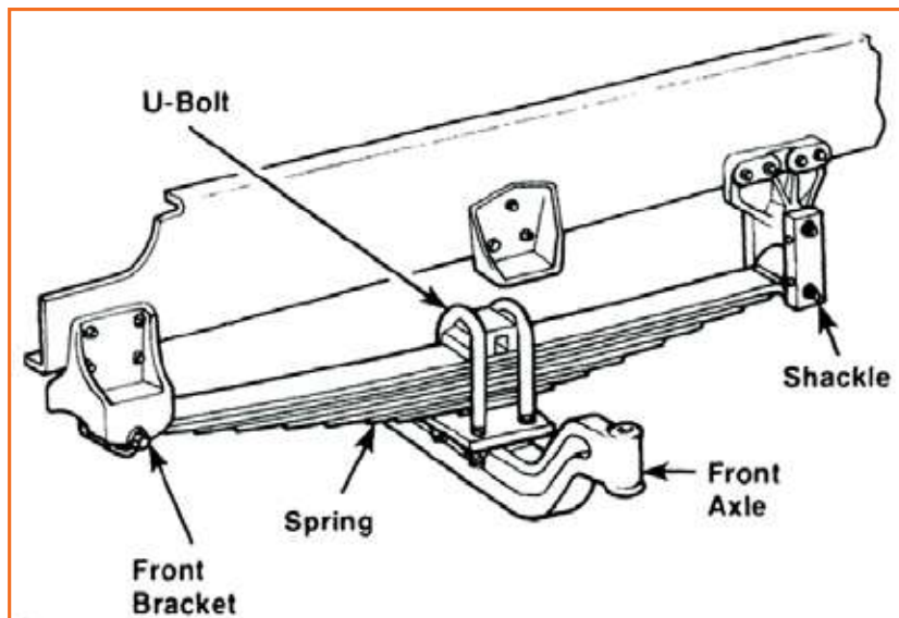
Fig 4.3.139: Spring pack
