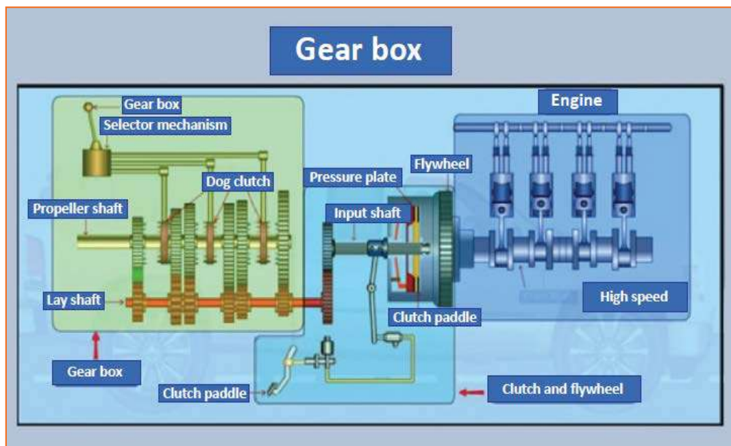
Fig 4.3.82: Gear box
