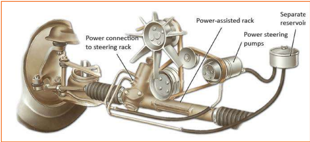
Fig 4.3.160: Steering rack in Power system
