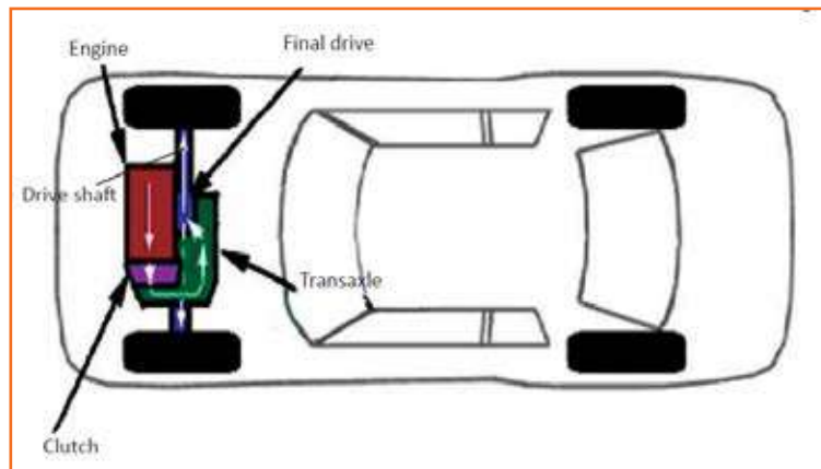
Fig 4.3.58: Front wheel drive
