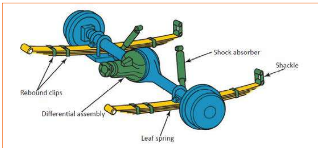
Fig 4.3.126: Typical rear leaf-spring suspension of a rear-wheel-drive vehicle
