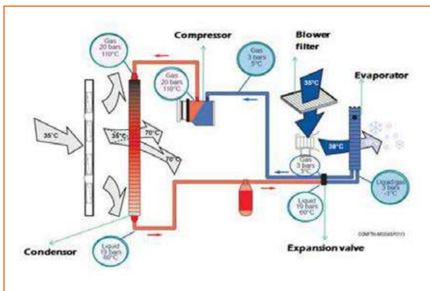
Fig 4.3.290: Working of air conditioning system
