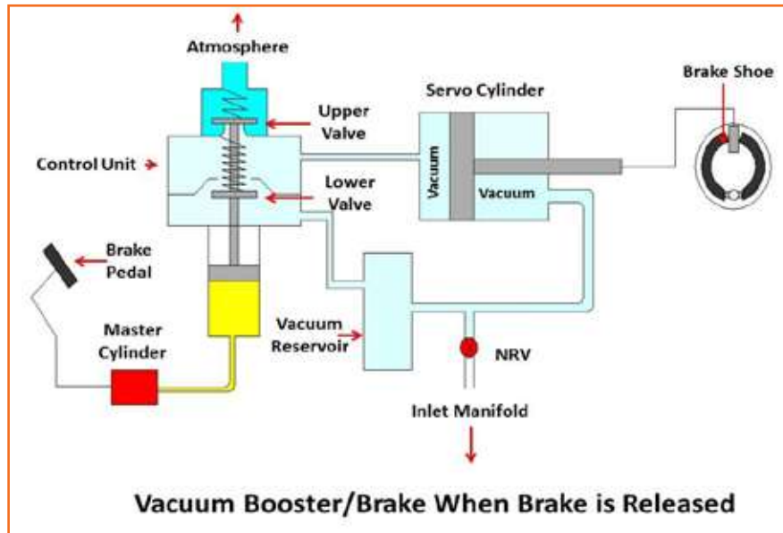
Fig 4.3.184: Master cylinder with vacuum Booster
