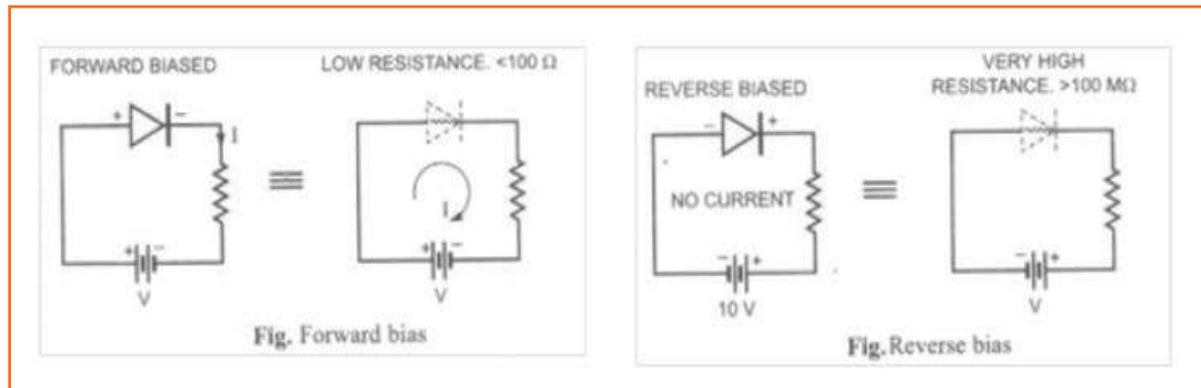
Fig 4.3.255: Biasing of Diodes
