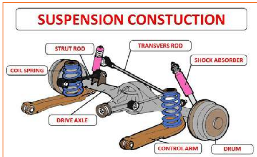
Fig 4.3.122: Parts of suspension system
