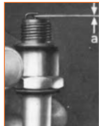
Fig 4.3.289: SPark plug
