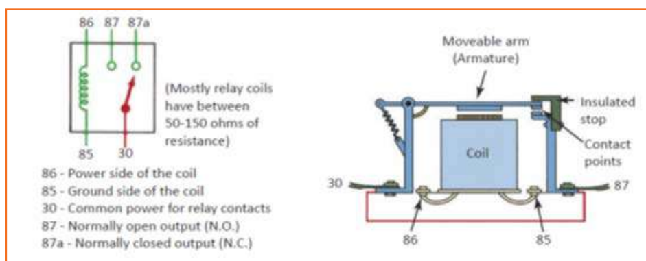
Fig 4.3.254: Relay cross-section view
