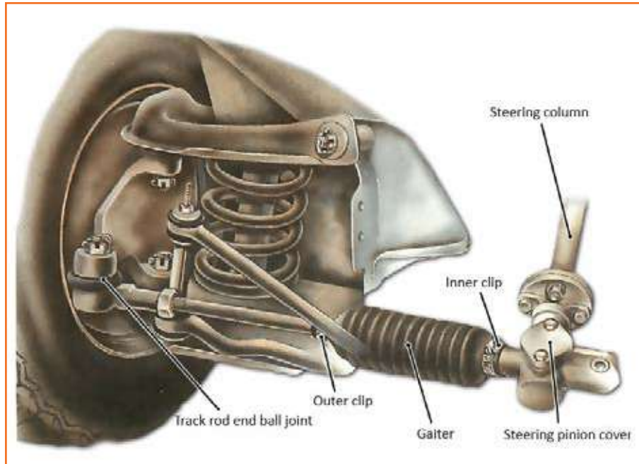
Fig 4.3.165: Rack & pinion steering
