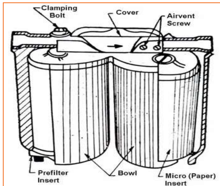
Fig 4.3.27: Duel filter assembly
