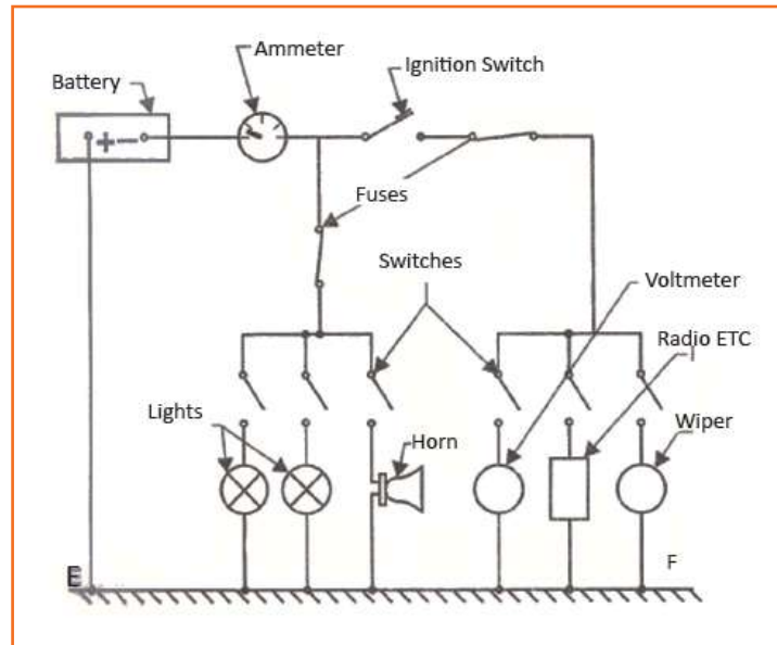
Fig 4.3.277: Lighting system diagram
