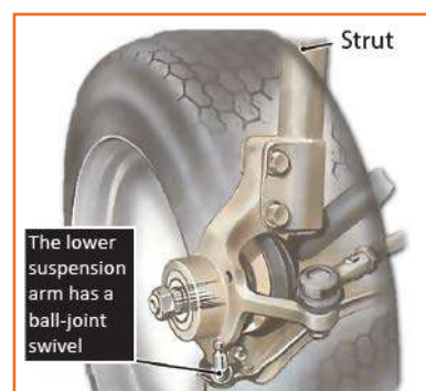
Fig 4.3.168: Macpherson strut
