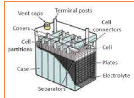
Fig 4.3.270: Battery
