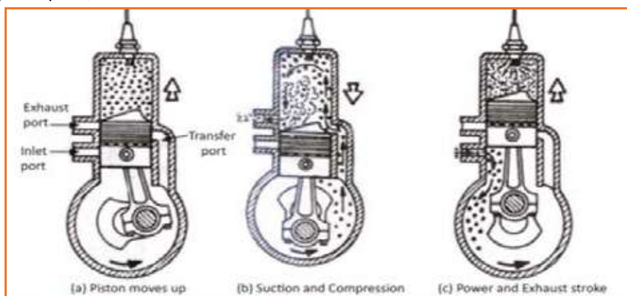
Fig 4.3.12: Two stroke engine
