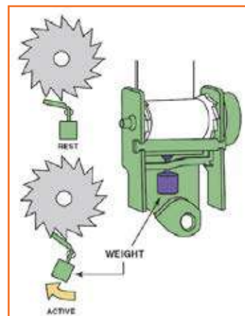
Fig 4.3.267: Locking mechanism
