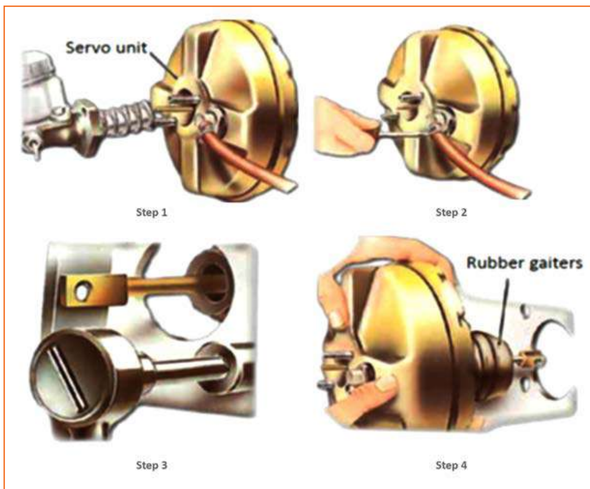
Fig 4.3.241: Replacing servo unit steps from 1 to 4
