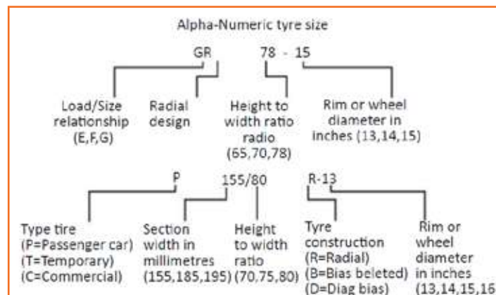
Fig 4.3.112: Tyre marking
