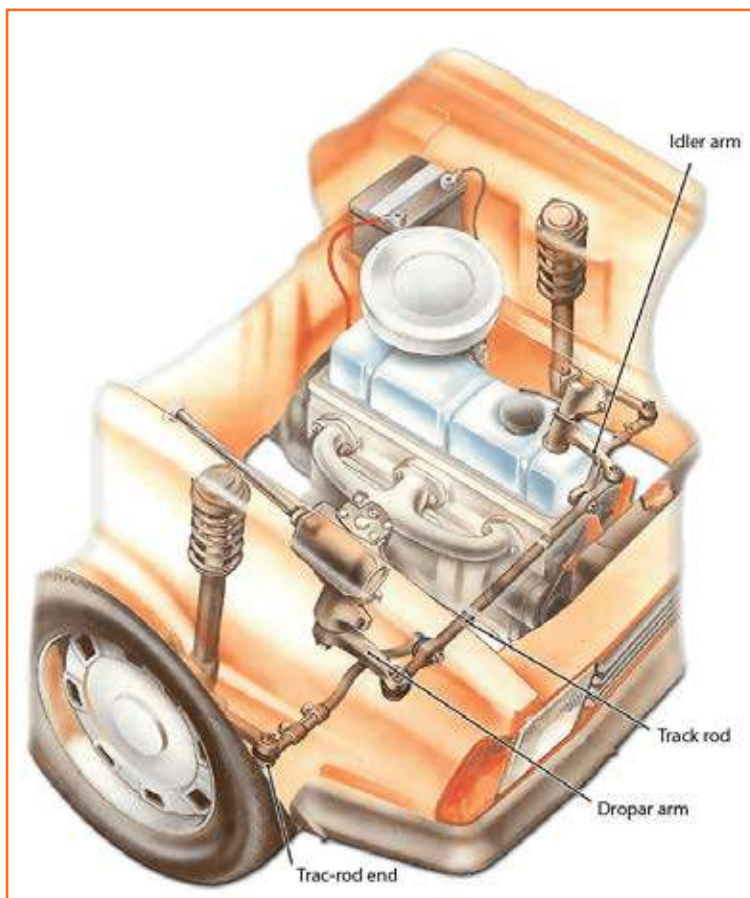
Fig 4.3.166: Steering-box system
