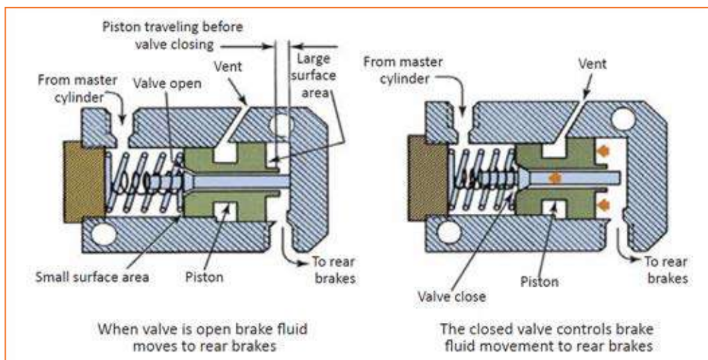
Fig 4.3.189: Working of PVC
