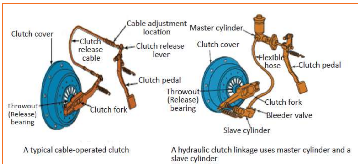
Fig 4.3.73: Types of clutches
