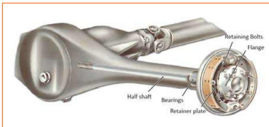
Fig 4.3.103: Half shaft check
