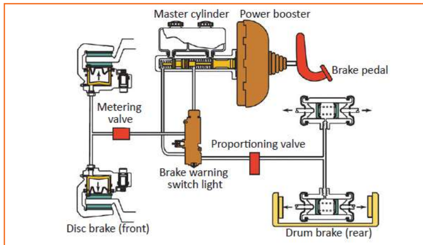
Fig 4.3.181: Components of brake system
