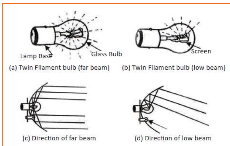
Fig 4.3.278: Headlights
