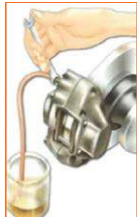
Fig 4.3.229: check the bleeding process 3
