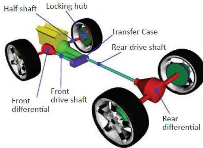
Fig 4.3.64: Four wheel drive
