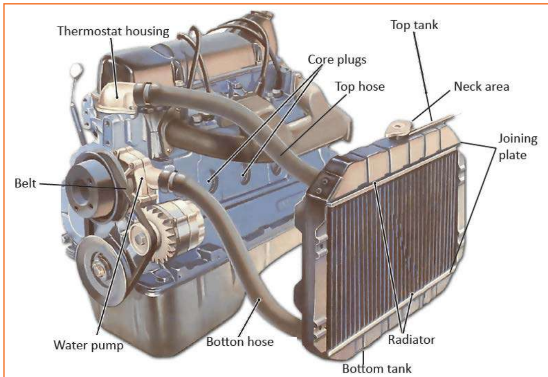
Fig 4.3.50: Water cooling system
