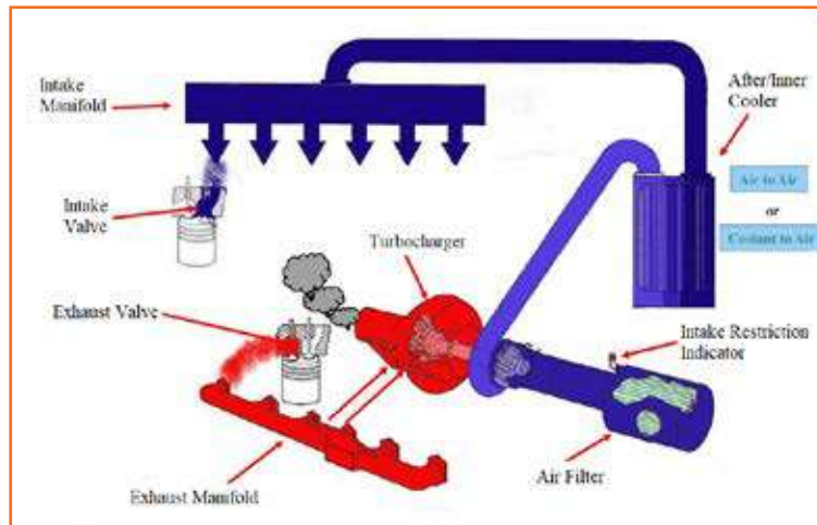
Fig 4.3.53: Air intake and exhaust system
