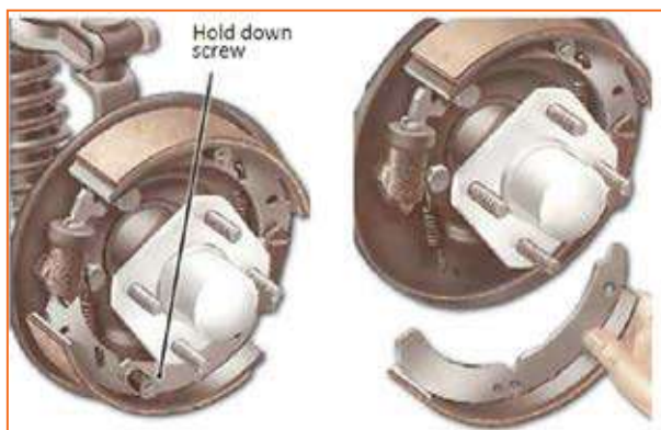
Fig 4.3.212: (A) Hold down spring (B) Removal brake shoe
