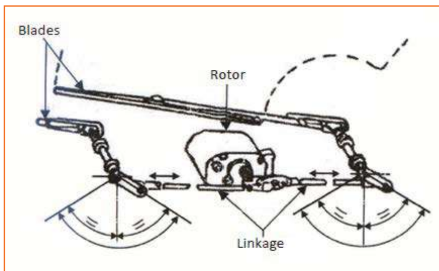
Fig 4.3.279: Wind shield wipers
