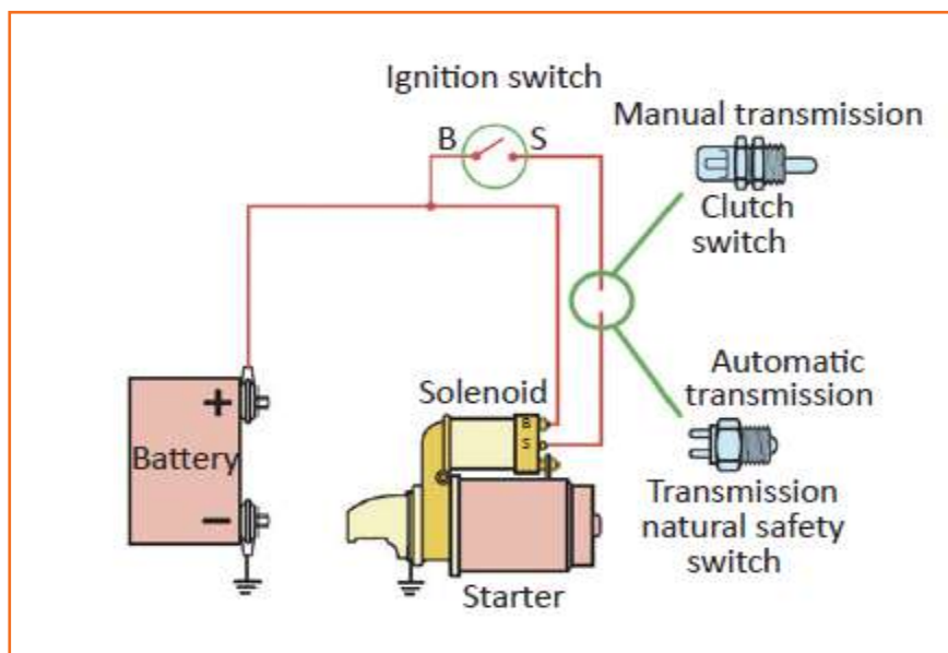
Fig 4.3.276: Starter motor function
