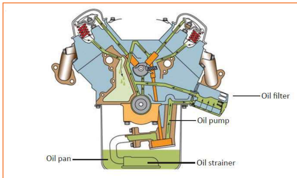
Fig 4.3.30: Lubrication system
