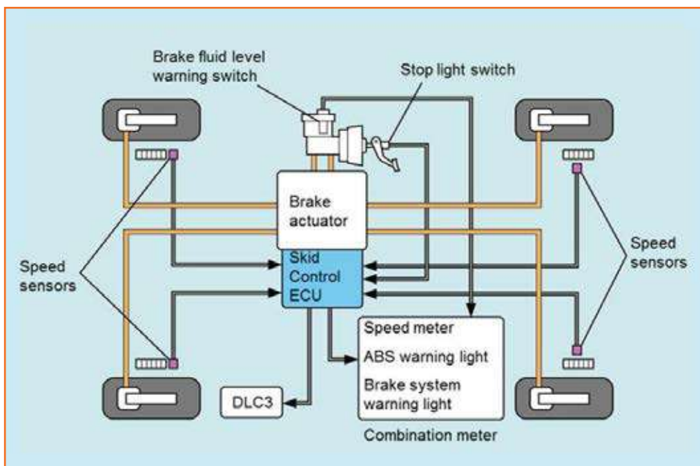
Fig 4.3.292: Skid control ECU
