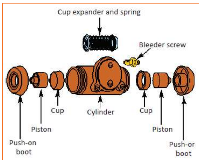
Fig 4.3.185: Wheel cylinder
