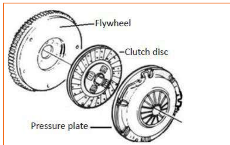
Fig 4.3.68: Clutch unit
