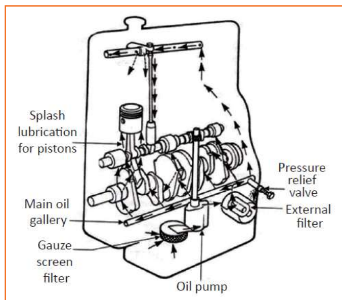
Fig 4.3.32: Engine parts require lubrication
