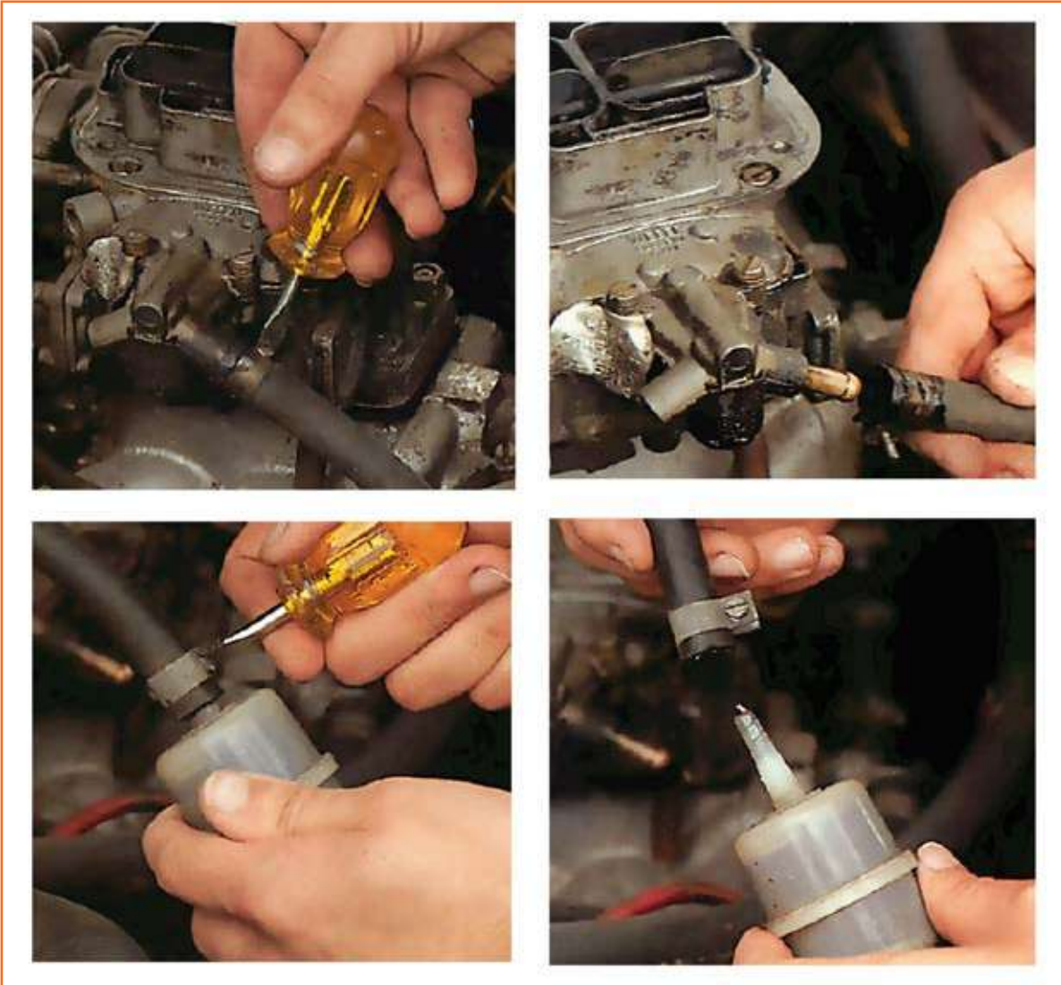
Fig 4.3.22: Replacing flexible fuel pipe
