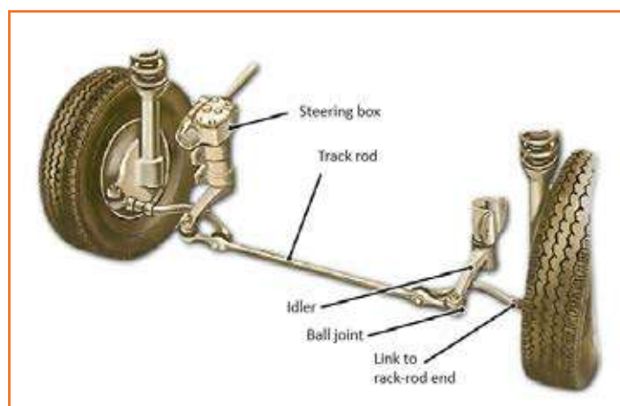
Fig 4.3.170: Steering-box system
