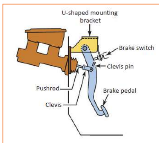
Fig 4.3.187: Master cylinder with vacuum Booster
