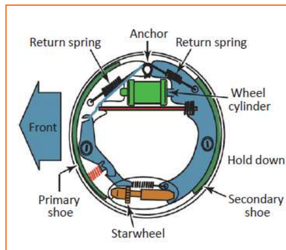
Fig 4.3.182: Drum brake
