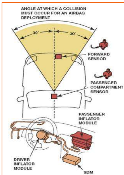
Fig 4.3.260: Air bag components
