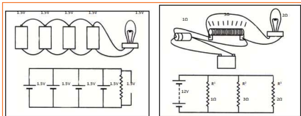
Fig 4.3.246: Parallel connection of storage cells & Resistors in parallel
