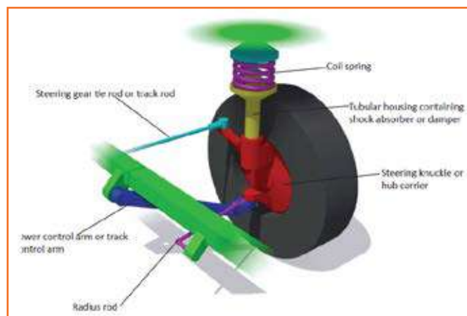
Fig 4.3.136: Mcpherson strut system
