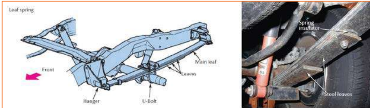
Fig 4.3.125: Leaf spring
