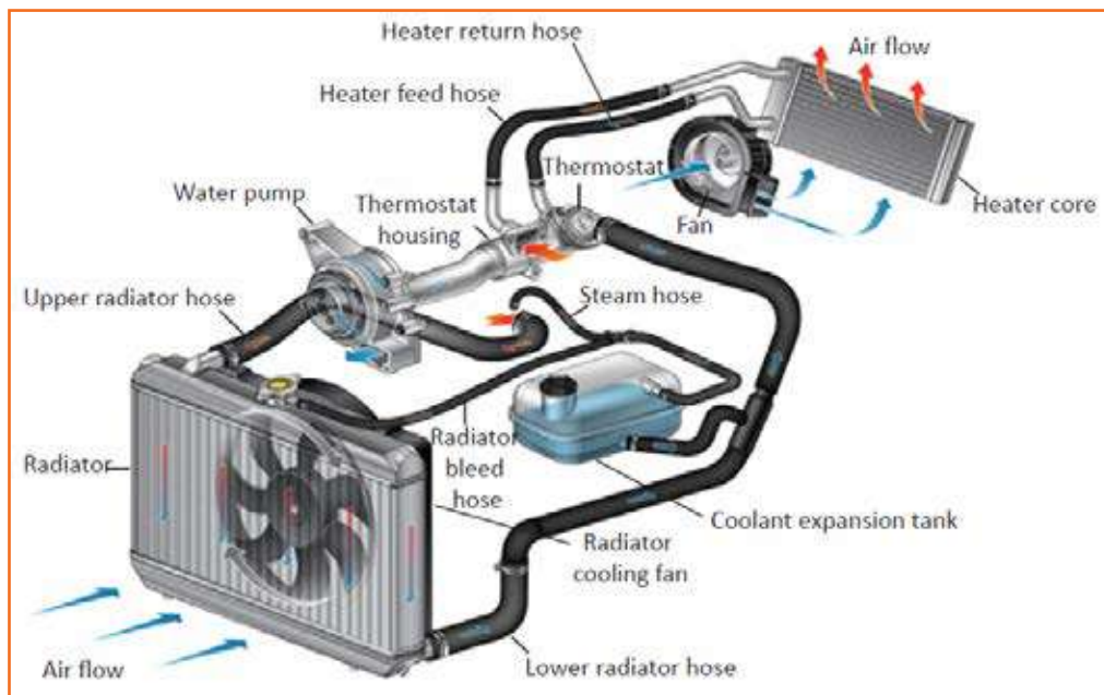
Fig 4.3.35: Engine cooling system
