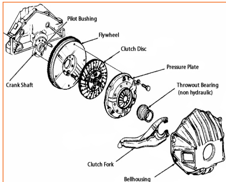
Fig 4.3.66: Components of the Clutch
