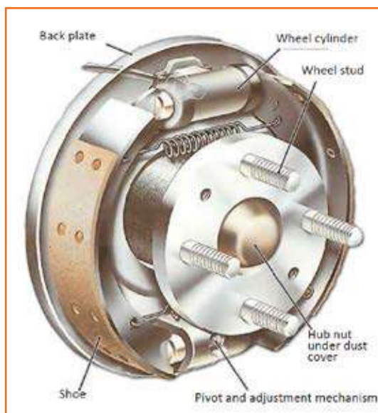
Fig 4.3.212: Leading and trailing shoe brake
