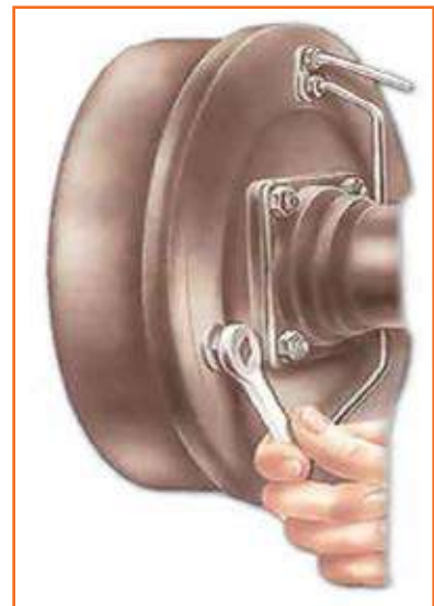
Fig 4.3.224: Adjusting snail cam
