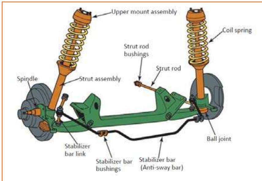
Fig 4.3.131: Stabilizer bars
