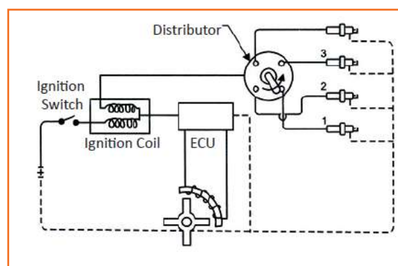
Fig 4.3.287: Ignition system
