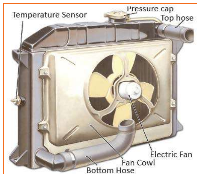
Fig 4.3.46: Car Radiator
