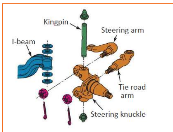
Fig 4.3.128: Steering knuckle
