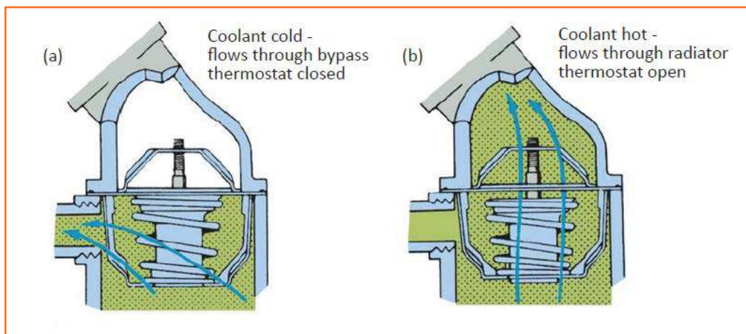
Fig 4.3.42: How thermostat works
