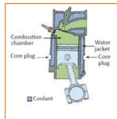
Fig 4.3.36: cooling unit
