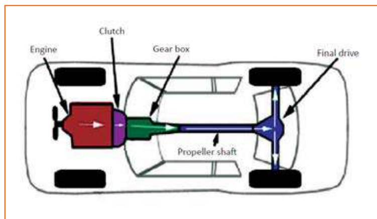
Fig 4.3.60: Rear wheel drive
