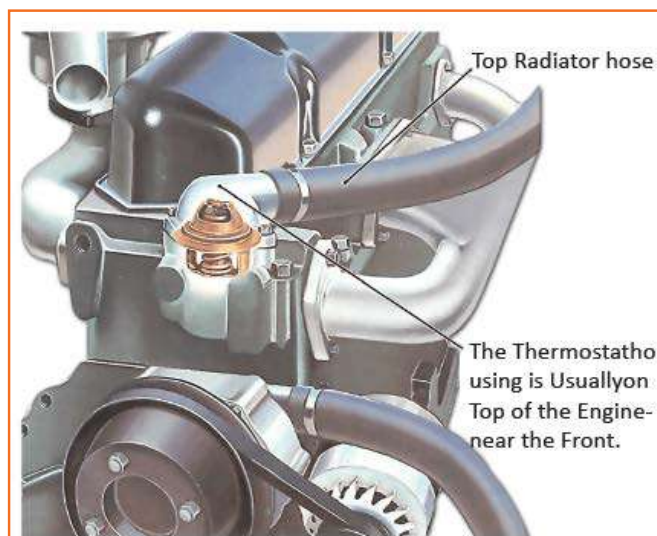
Fig 4.3.43: Thermostat testing
