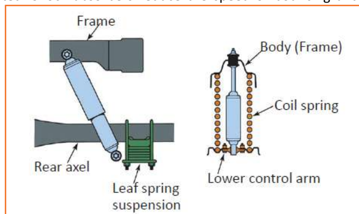
Fig 4.3.133: Shock absorbers
