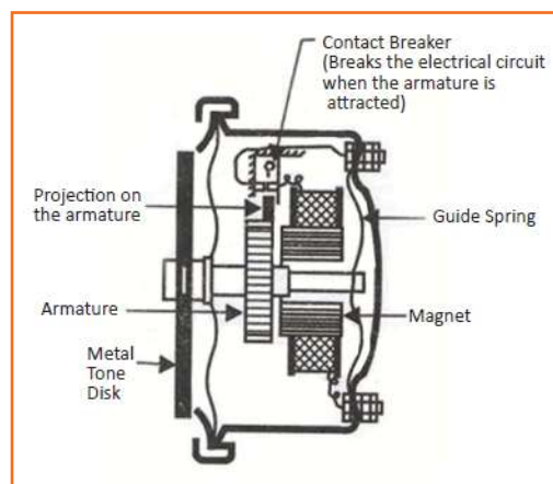
Fig 4.3.280: Electric horn working
