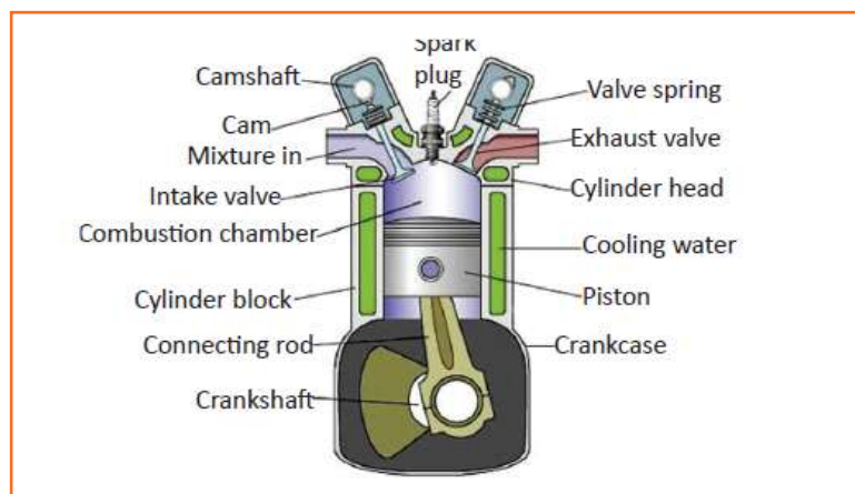
Fig 4.3.1: Components of an Engine
