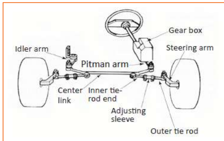
Fig 4.3.145: Components of steering system
