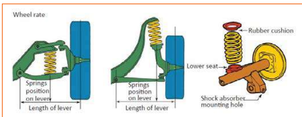
Fig 4.3.124: Coil spring
