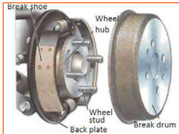
Fig 4.3.203: Separate drum brake
