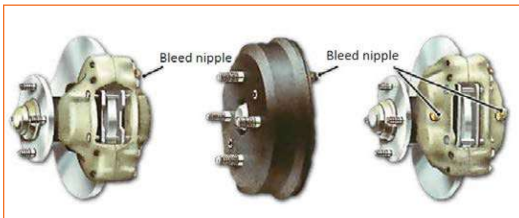
Fig 4.3.226: Location bleed nipples
