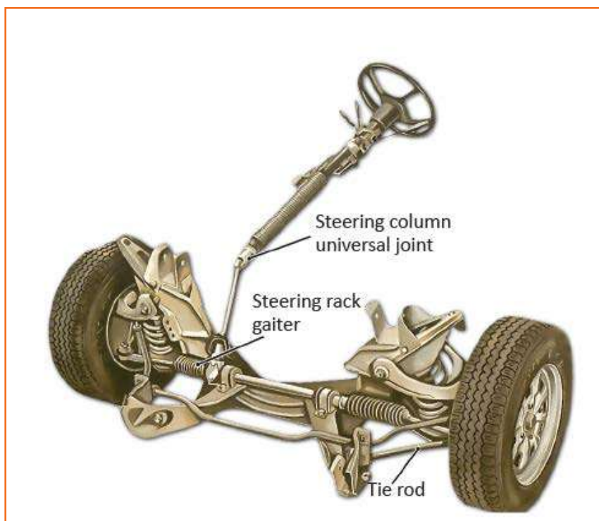
Fig 4.3.171: Steering-rack system
