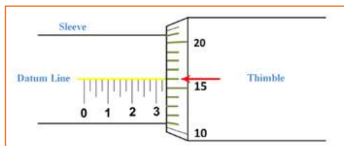
Fig 4.2.26: Micrometer scale
