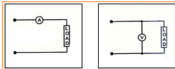
Fig 4.3.247: Ammeter in series & Voltmeter in parallel
