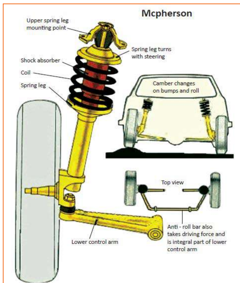
Fig 4.3.138: Mcpherson Strut System
