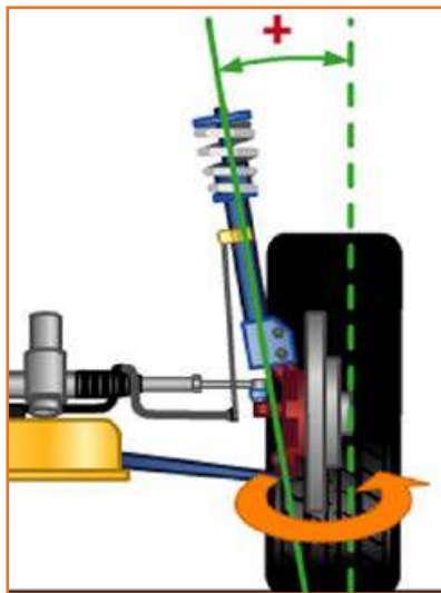
Fig 4.3.175: King Pin Inclination
