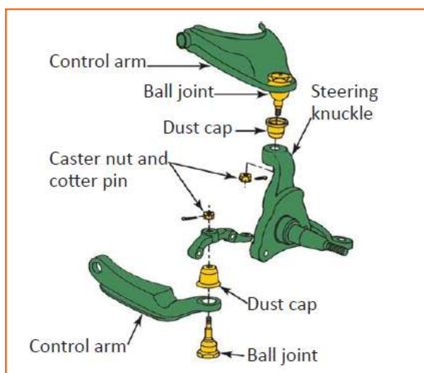
Fig 4.3.129: Control arm
