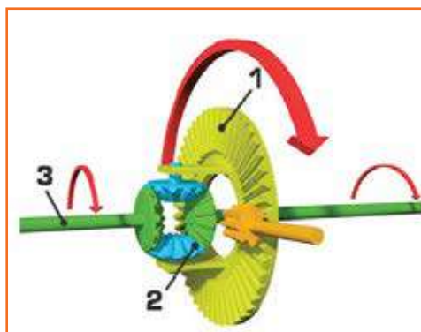
Fig 4.3.95: Differential working
