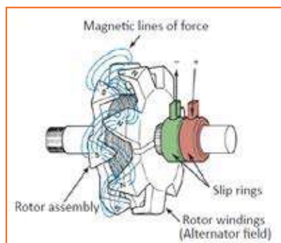
Fig 4.3.274: Alternator
