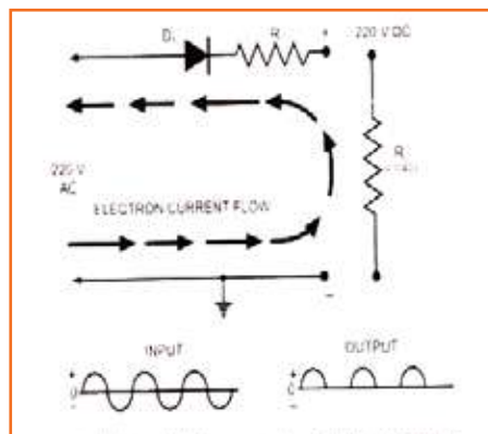
Fig 4.3.257: DC power supply
