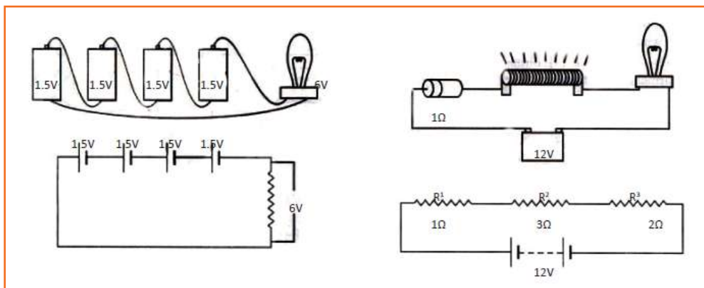
Fig 4.3.245: Series connection of storage cells
