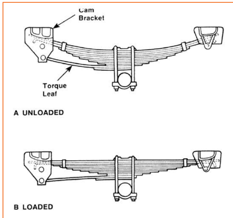
Fig 4.3.140: Progressive spring operation
