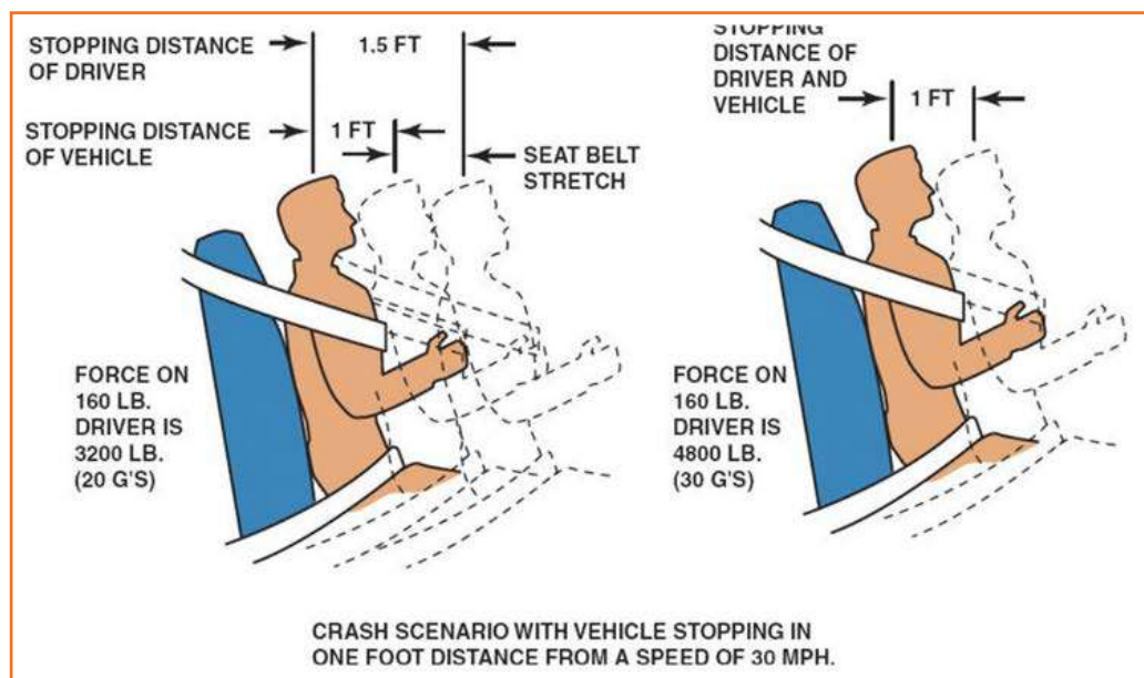
Fig 4.3.266: Seat belt crash scenario working
