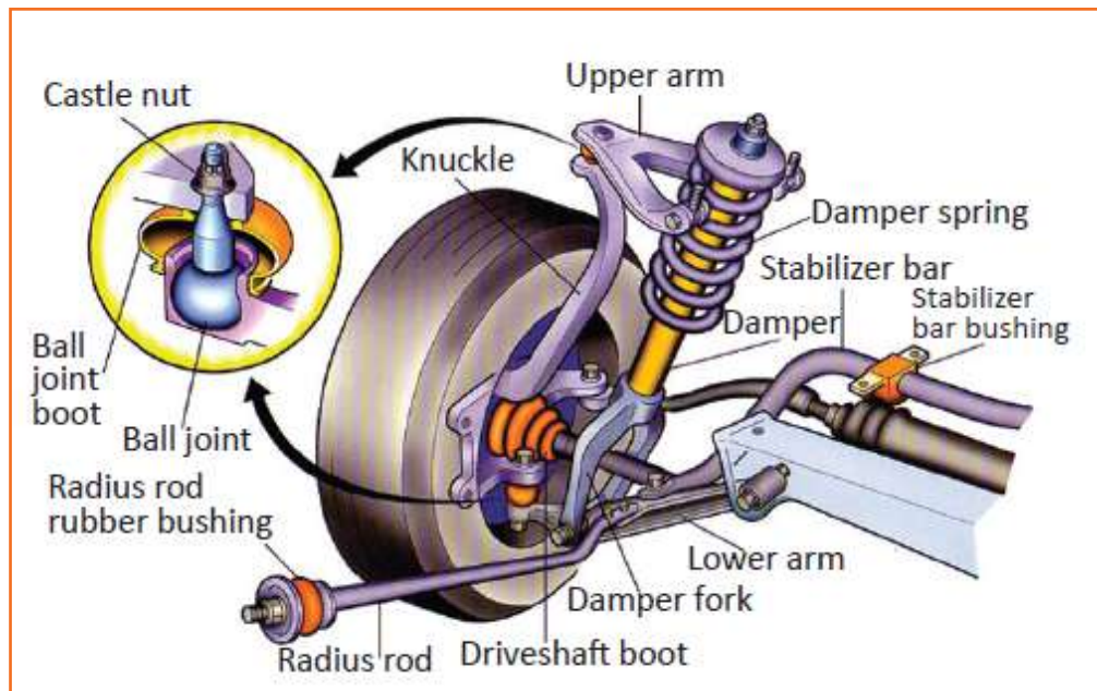
Fig 4.3.137: Mcpherson strut system
