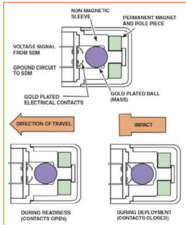
Fig 4.3.262: Airbag magnetic sensor
