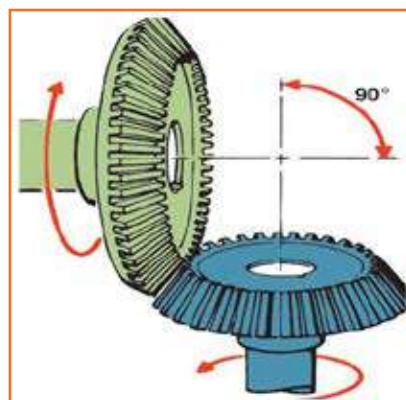
Fig 4.3.101: Axle ratio
