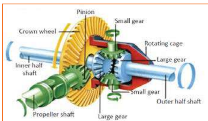
Fig 4.3.96: Differential assembly
