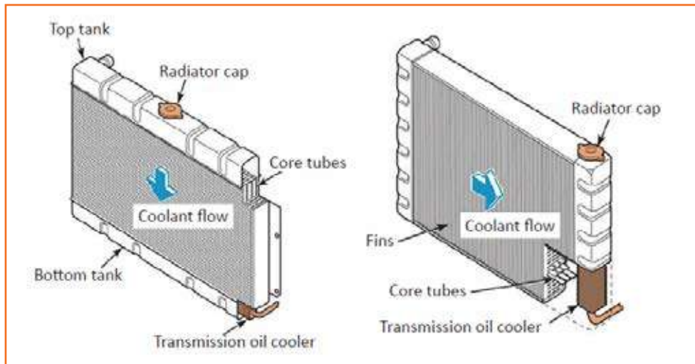
Fig 4.3.38: Radiator
