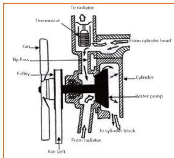
Fig 4.3.40: Fan, water pump and thermostat
