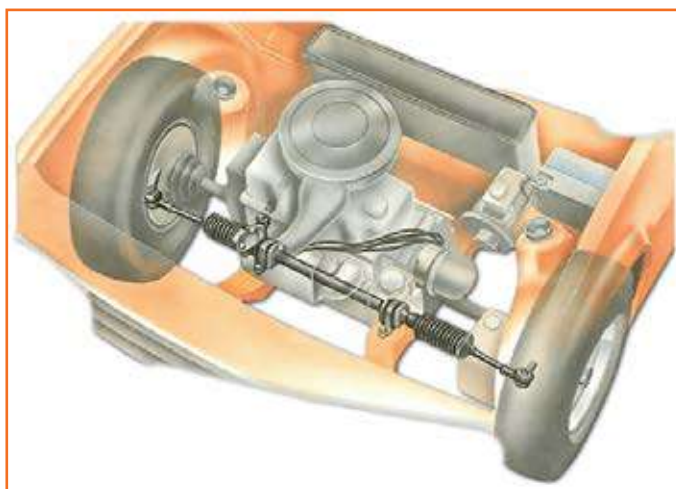
Fig 4.3.162: Power steering rack
