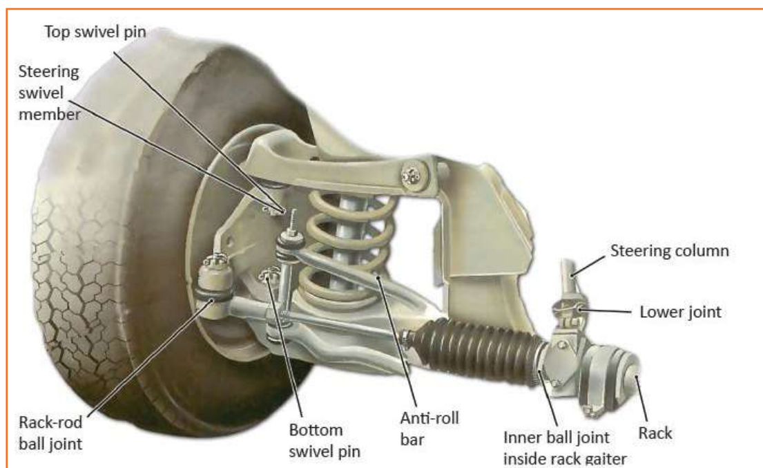
Fig 4.3.178: Lubricating the steering system
