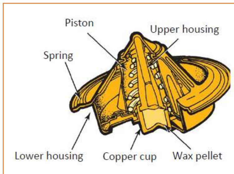
Fig 4.3.41: Thermostat
