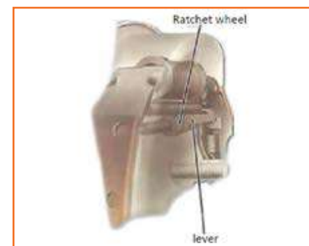
Fig 4.3.219: Automatic adjuster
