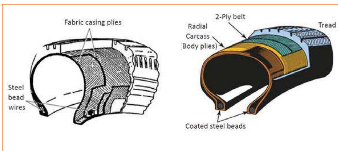
Fig 4.3.108: Tyre 1 & Tyre 2
