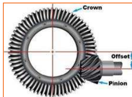
Fig 4.3.100: Hypoid drive
