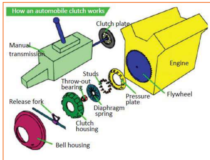
Fig 4.3.67: Components of the Clutch
