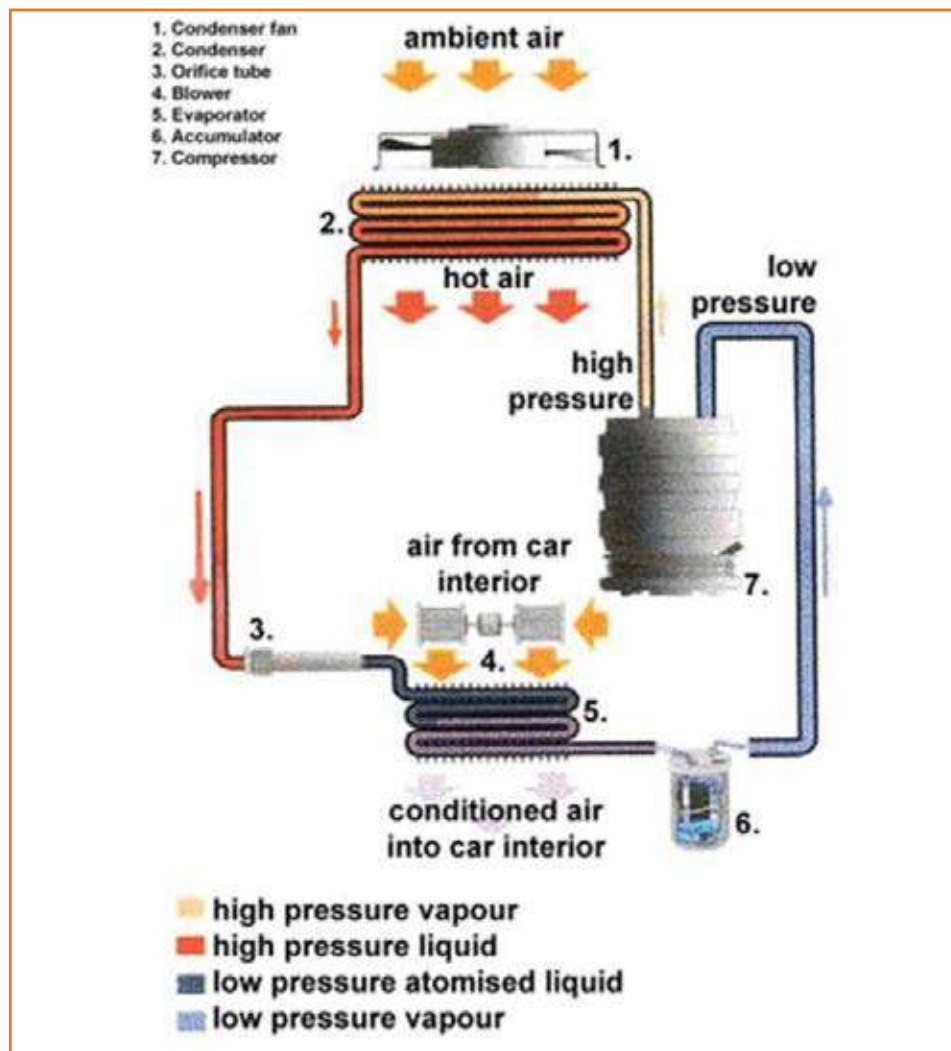
Fig 4.3.289: Air conditioning system
