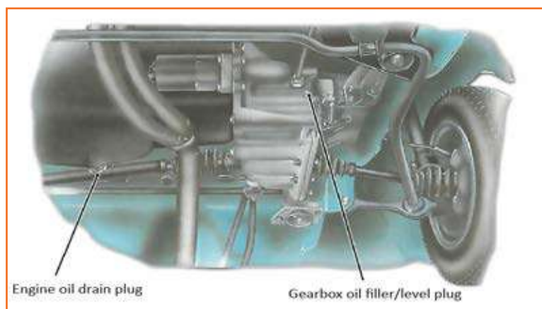
Fig 4.3.88: Layout under a transverse-engine front-wheel-drive car
