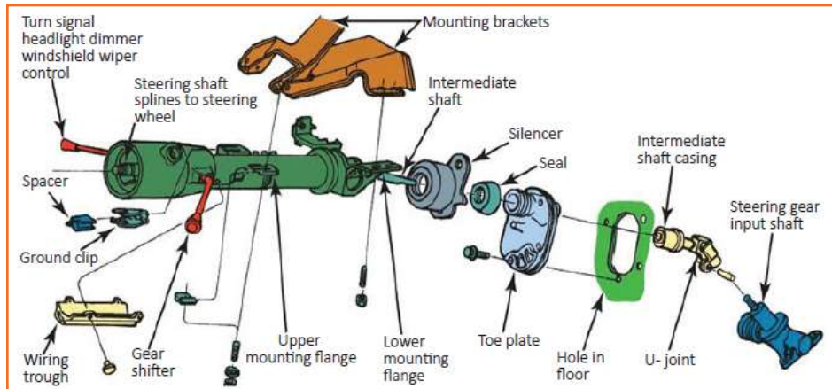
Fig 4.3.147: Components of steering column
